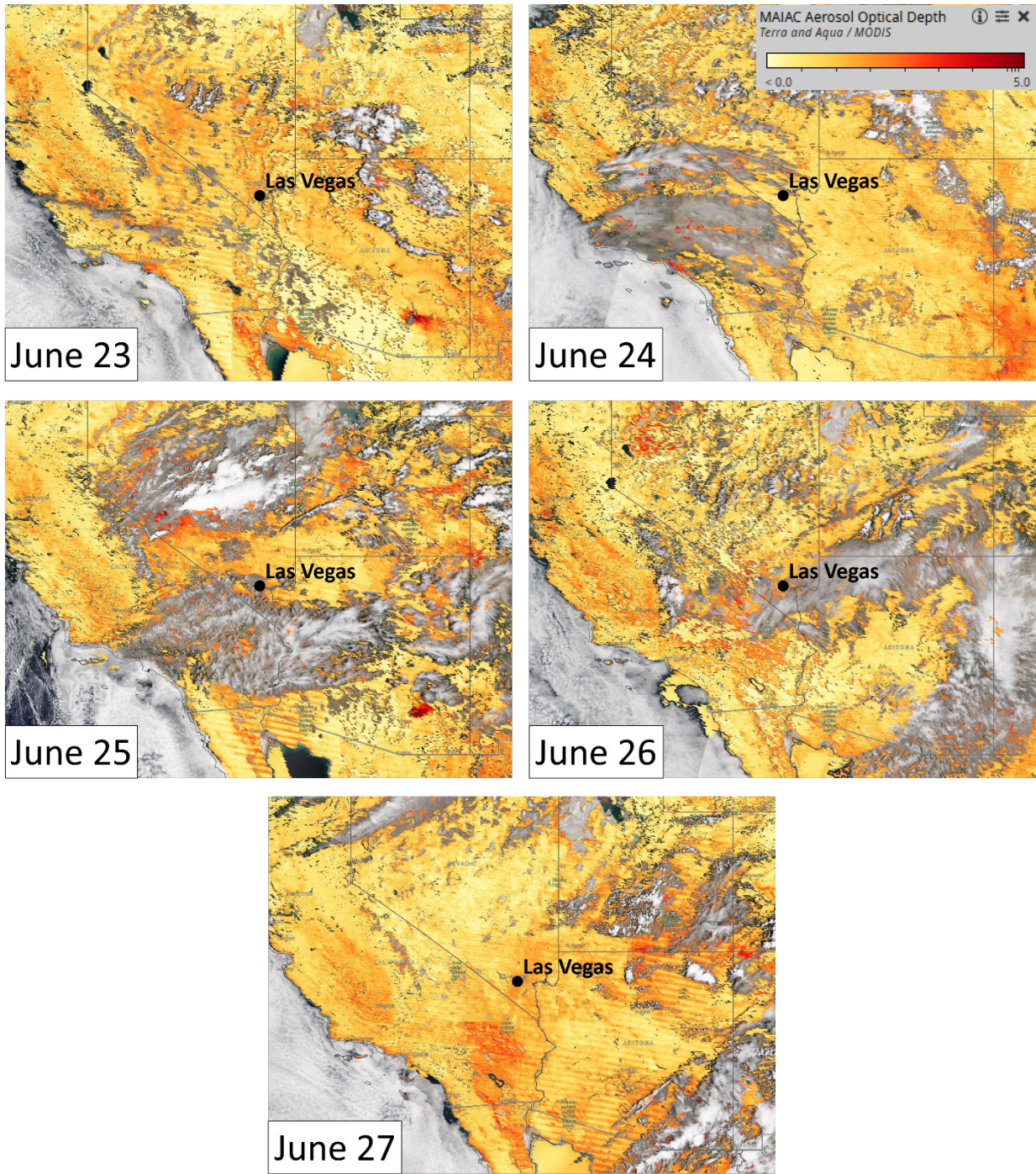
Figure B-1. MAIAC MODIS Aqua/Terra combined AOD retrievals June 23 – 27, covering the three days before the exceptional event, the day of the event (June 26), and the day after the event. AOD color ranges from yellow (low AOD) to red (high AOD).
