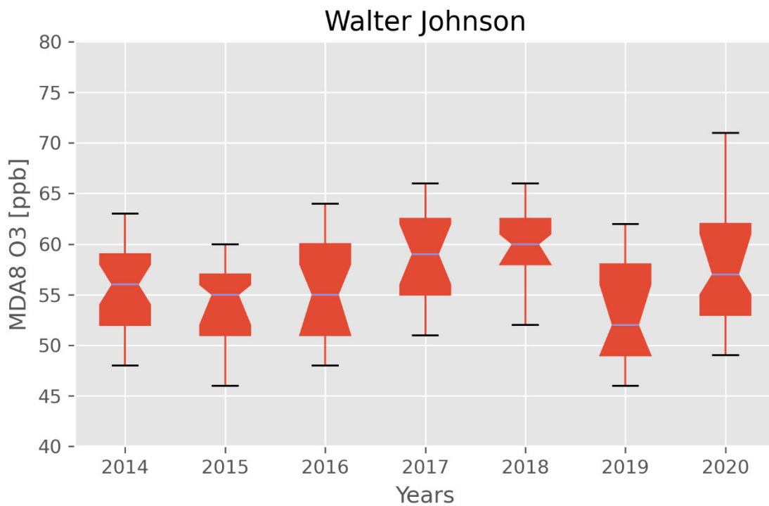
Figure G-2. Annual May distributions of MDA8 ozone at sites with exceptional events during May 2020. Notches denote 95 th confidence interval of the median, boxes are 25 th , 50 th and 75 th percentiles, and whiskers are 5 th and 95 th percentiles.
